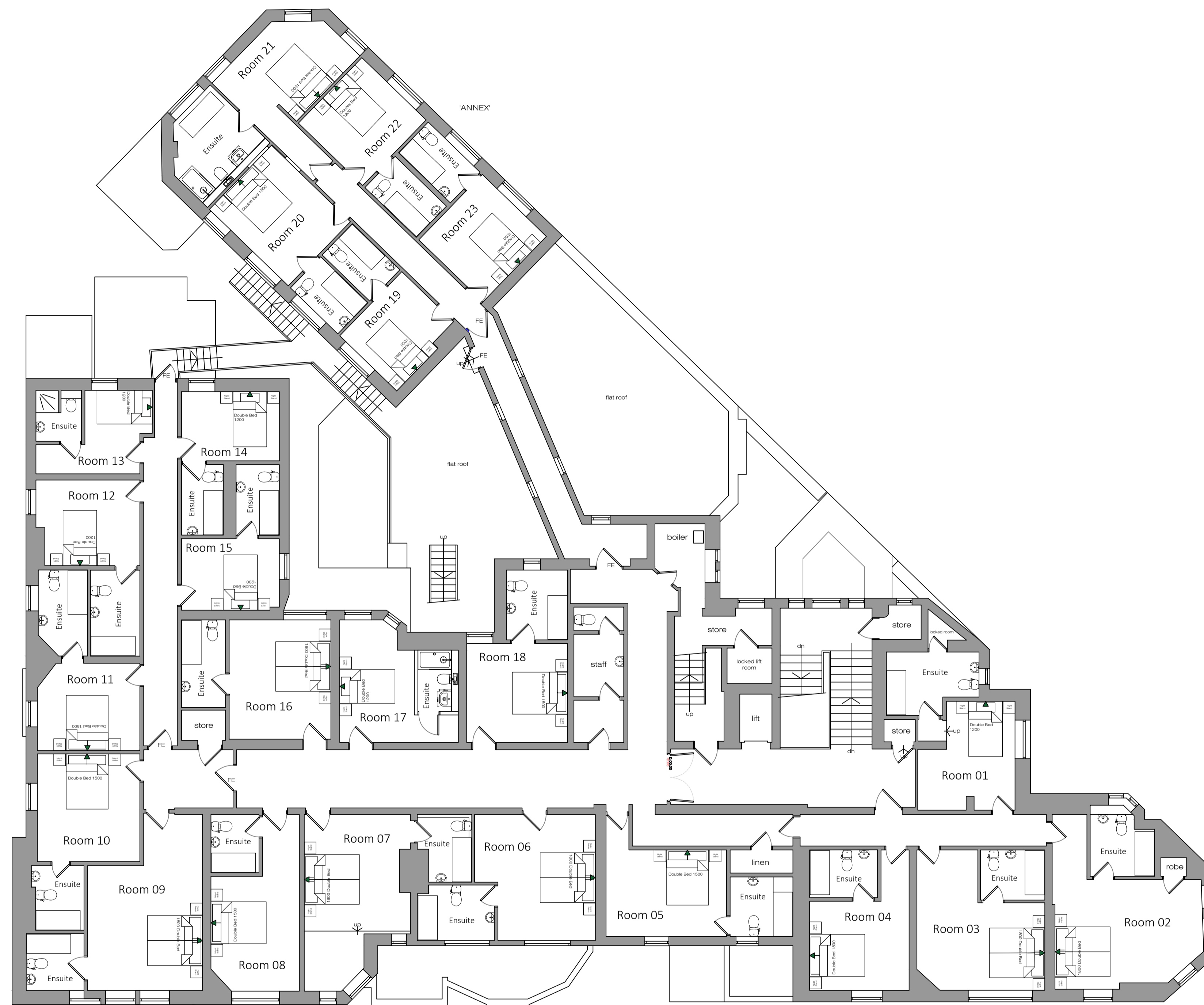
First Floor
